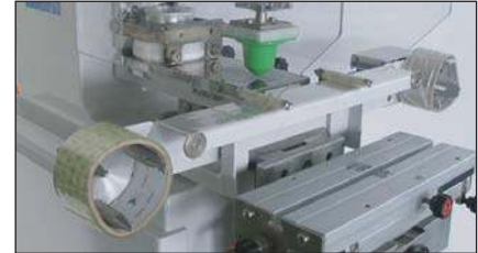
Automatic pad clean between work table and printing platform
